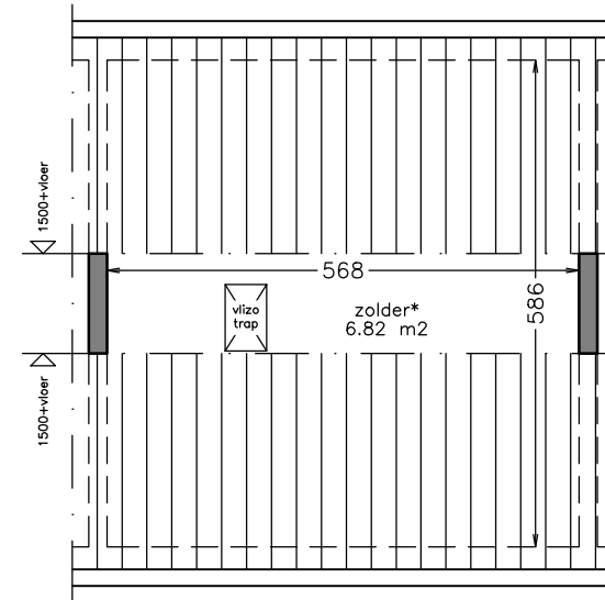
zolder
